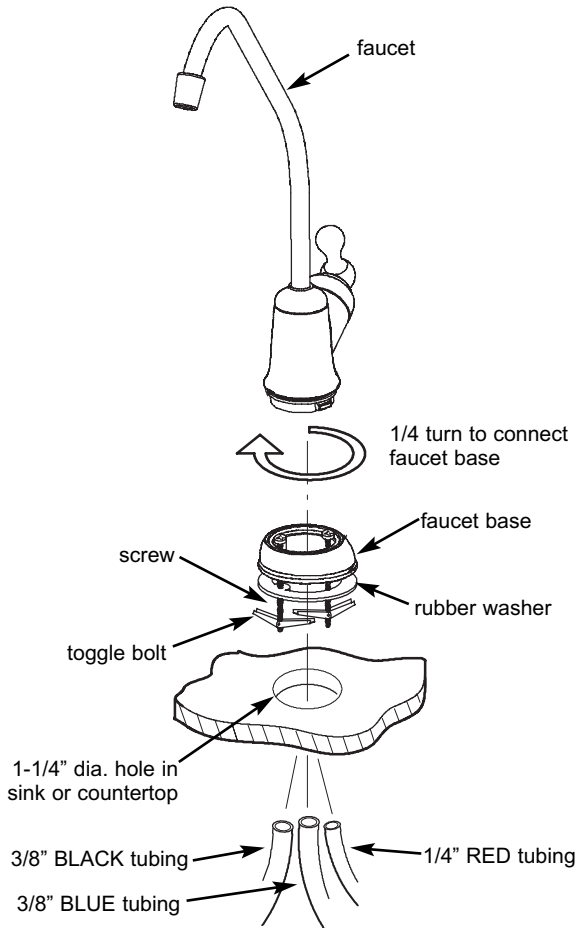
FIGURE 3 - FAUCET INSTALLATION
